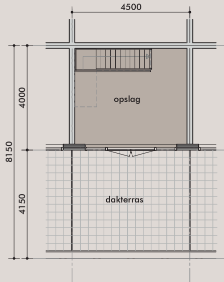
1 e verdieping 18,0 m 2
