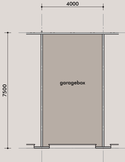
Begane grond 30,0 m 2
