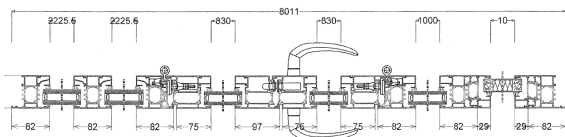
horizontale detail
